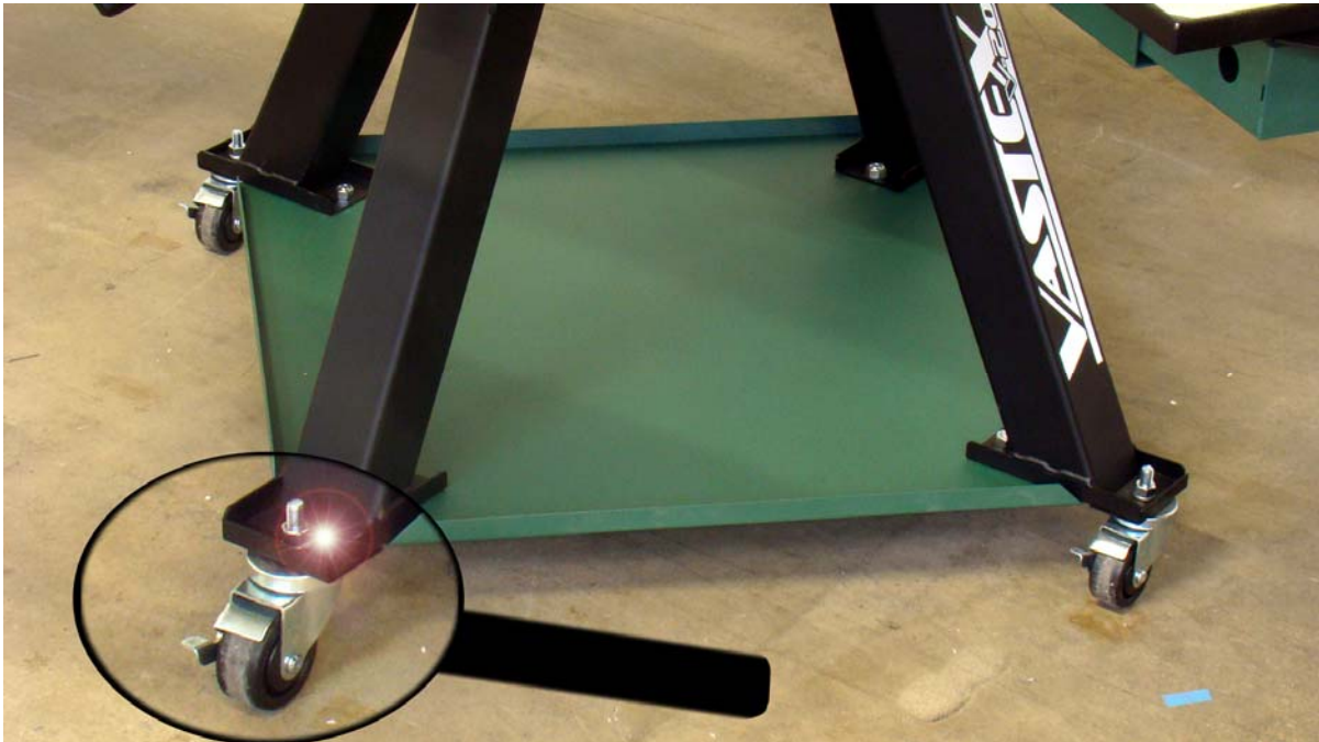
V-2000 Service Pan and Wheels (shown above) raise machine height 4.25". Wheels are available without Service Pan.
